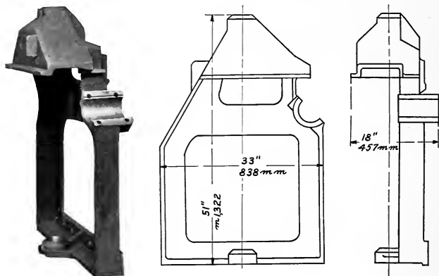
Fig. 73. Side Frame Casting.
